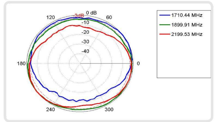
Port 2 Vertical: 1700 - 2200
