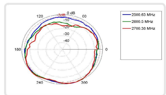
Port 2 Vertical: 2500 - 2700
